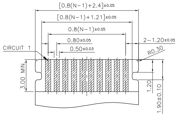
APPLICABLE FPC (THICKNESS: 0.2±0.03)
